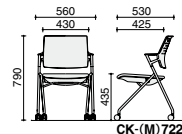
CK-(M)722
