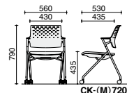
CK-(M)720
